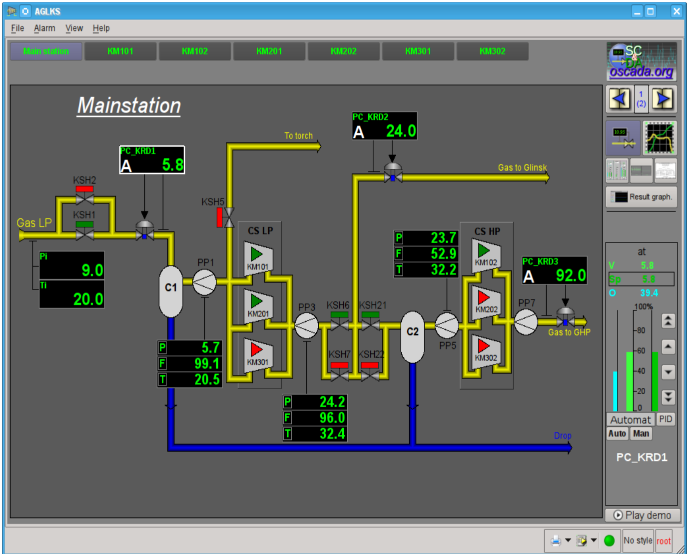
Fig.3. The main window if the execution mode.
