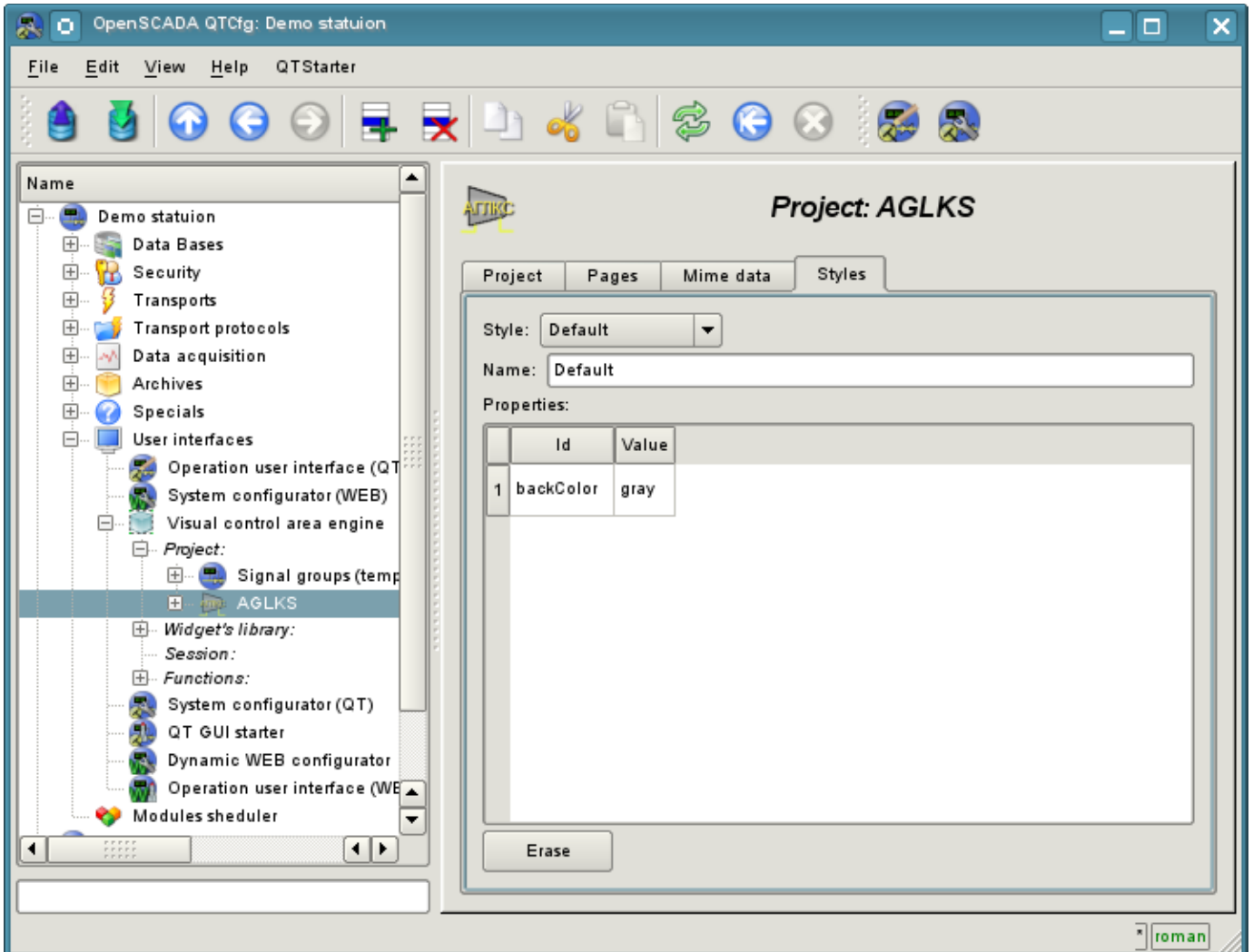
Fig. 3.3 "Styles" tab of the configuration page of the project.
