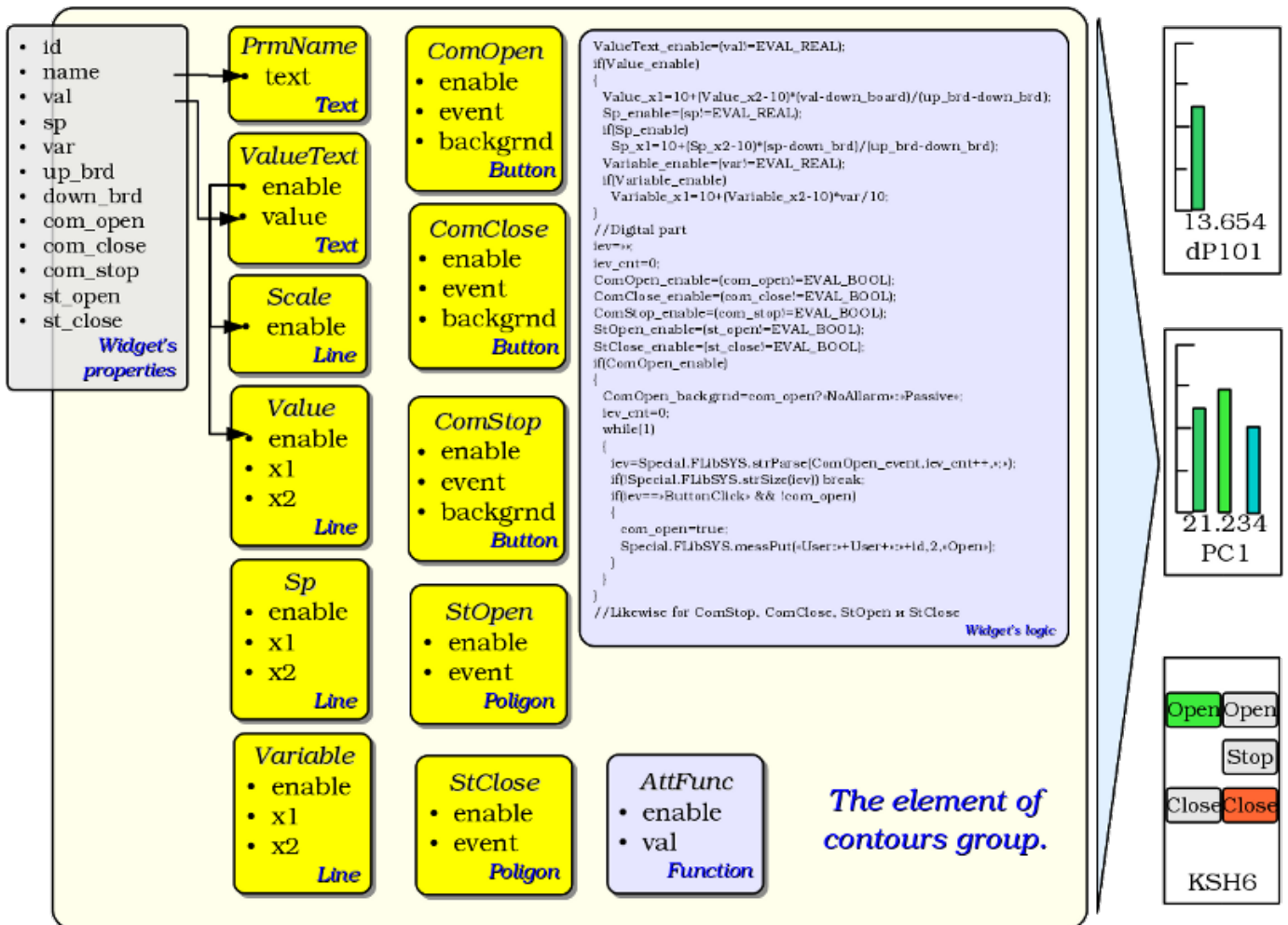
Fig.3.1.1 Example of the structure of the derived widget.
