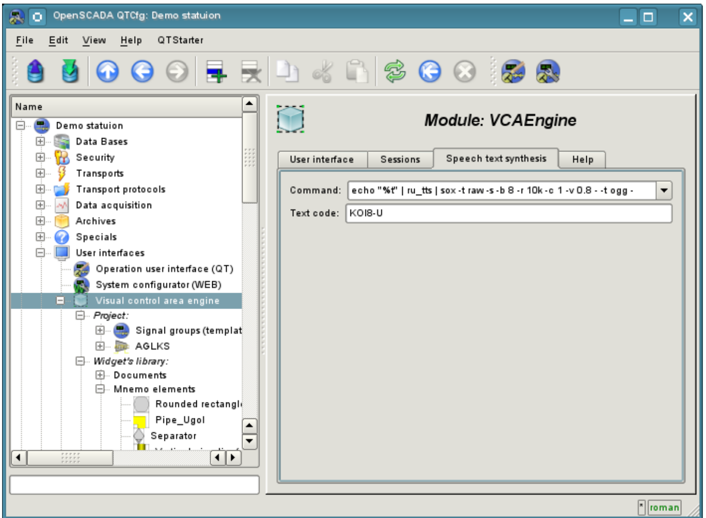
Fig.4.3 The inset for speech synthesis engine configuration.
