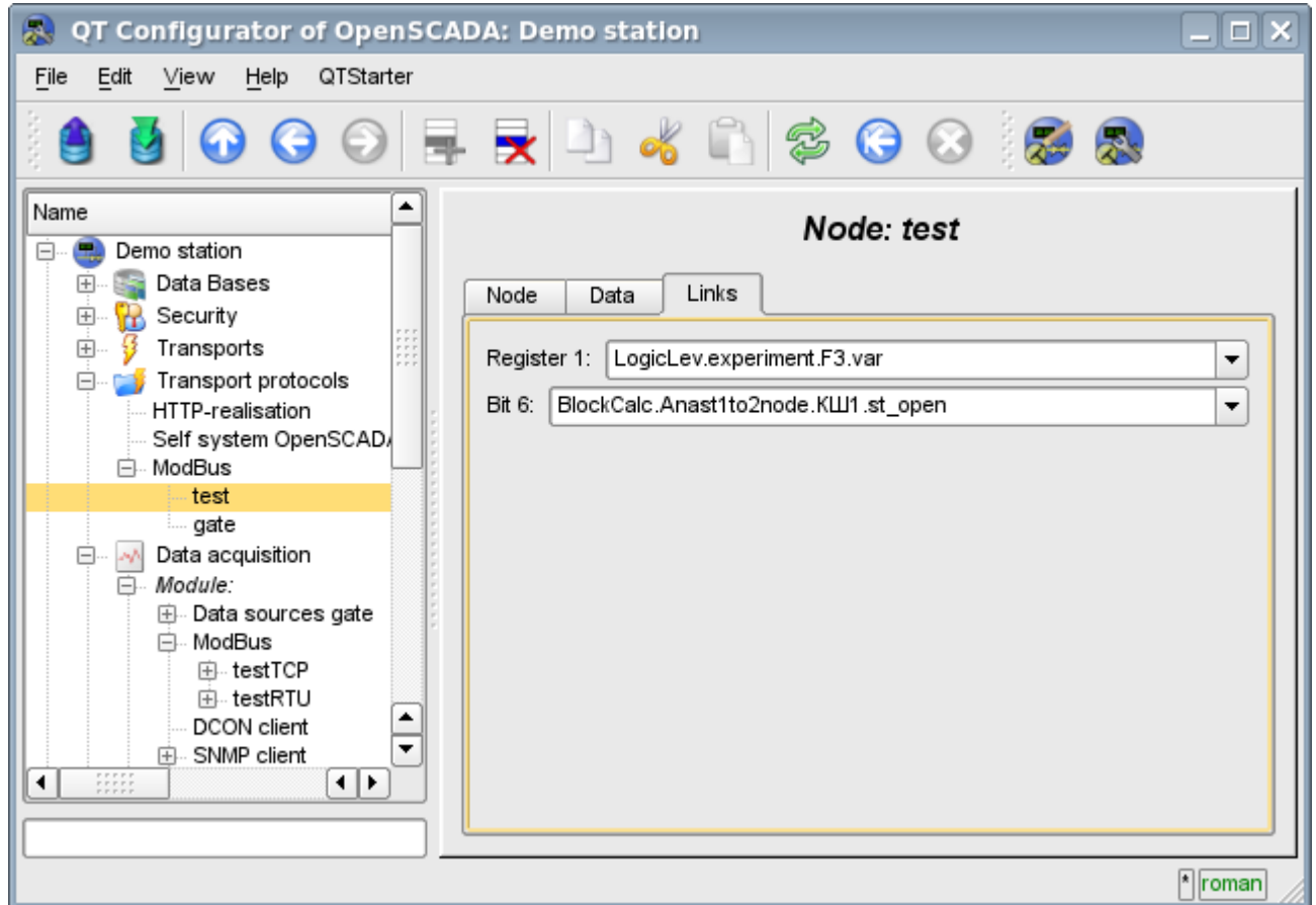
Fig.4. The tab “Links” of the configuration page of the node of the protocol in the “Data” mode.
